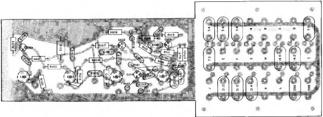
FIGURE 7-5 X-RAY VIEW, RF MODULE
