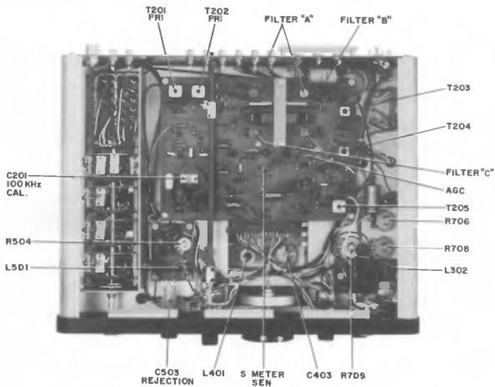
FIGURE 4-2 BOTTOM VIEW OF HQ-215
