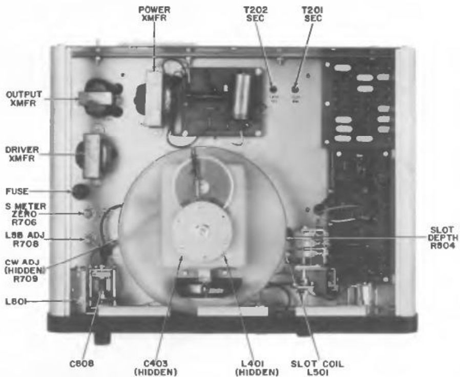
FIGURE 4-1 TOP VIEW OF HQ-215
