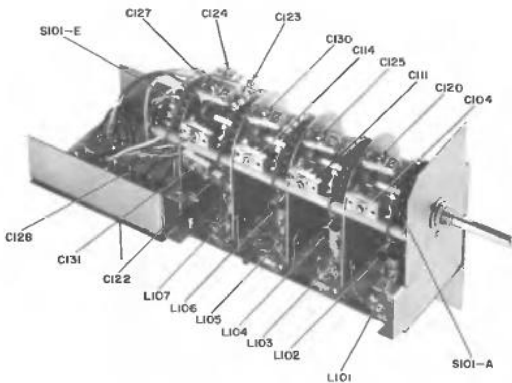
FIGURE 4-3 RF MODULE WITH BANDSWITCH
