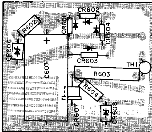
FIGURE 7-4 X-RAY VIEW, POWER SUPPLY MODULE
