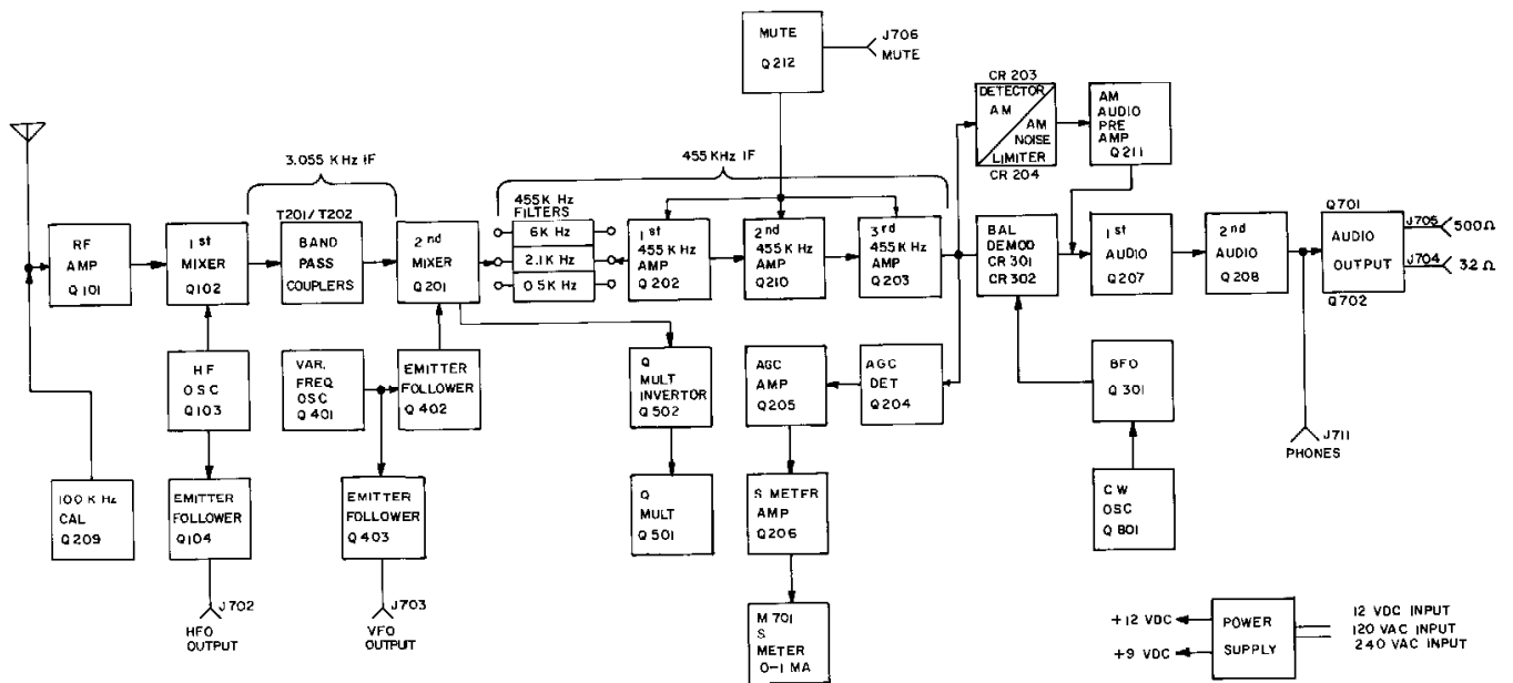
FIGURE 7-7 BLOCK DIAGRAM
