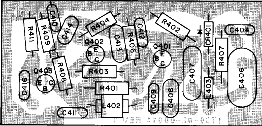
FIGURE 7-3 X-RAY VIEW, VFO MODULE
