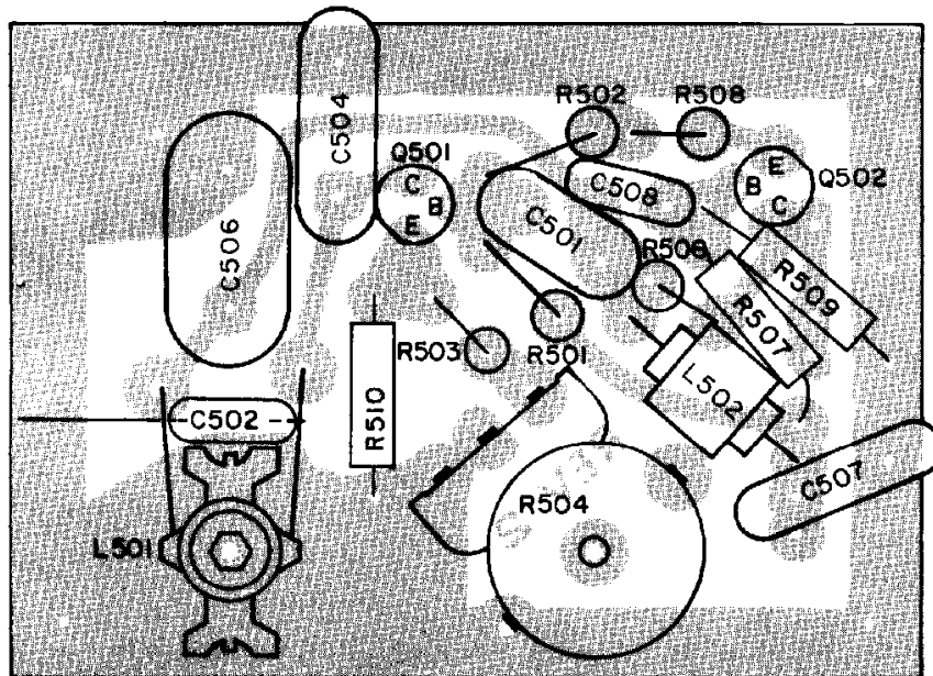
FIGURE 7-1 X-RAY VIEW, SLOT FILTER MODULE
