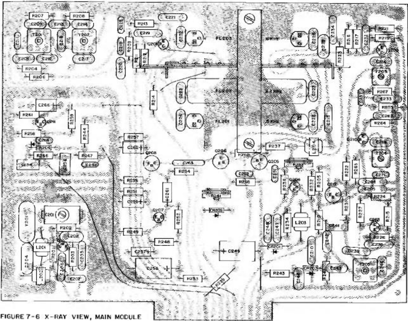
FIGURE 7-6 X-RAY VIEW, MAIN MODULE
